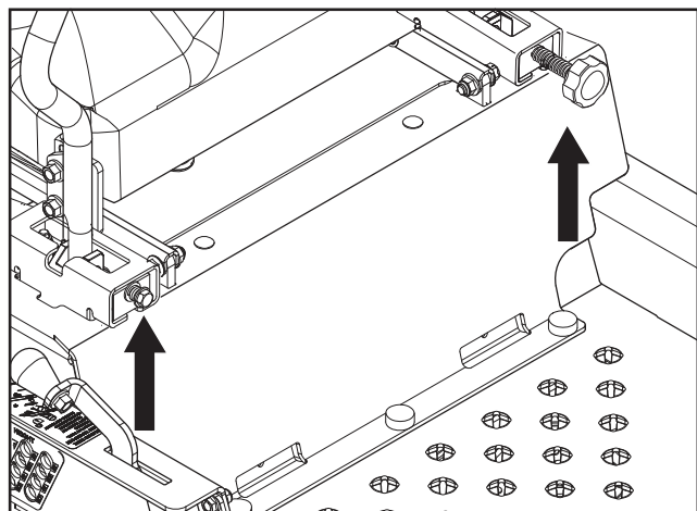
Tracking adjustment
