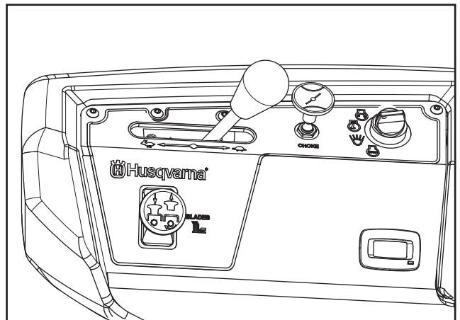
Choke control
